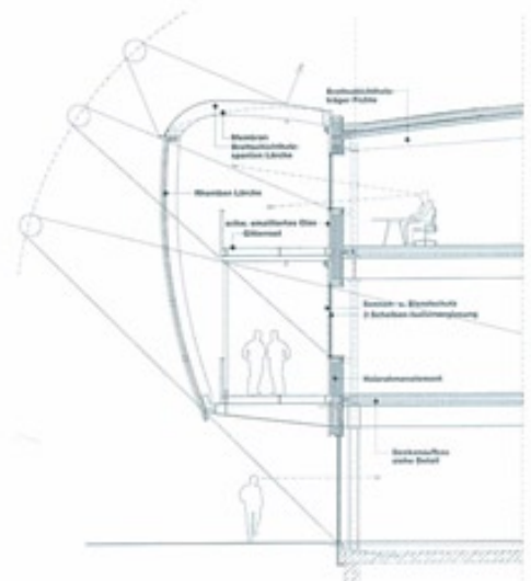
Fassadendetail Detail facade
